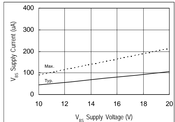
Figure 12B. V_{BS} Supply Current vs. Supply Voltage
