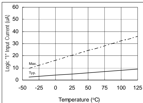
Figure 14A. Logic "1" Input Current vs. Temperature
