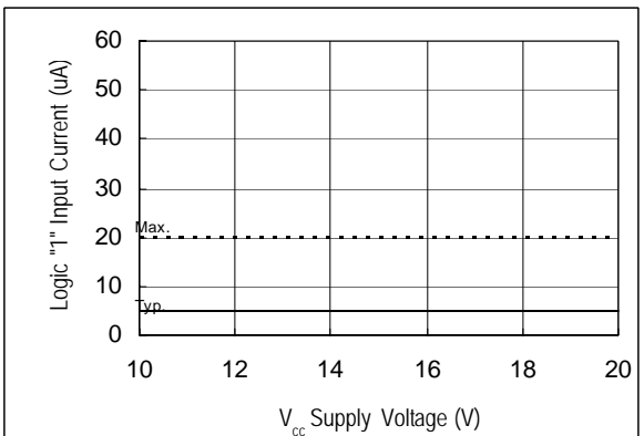
Figure 14B. Logic "1" Input Current vs. Supply Voltage
