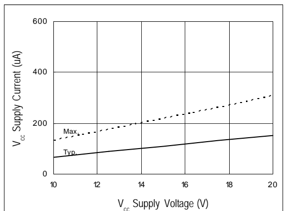
Figure 13B. V_{CC} Supply Current vs. Supply Voltage
