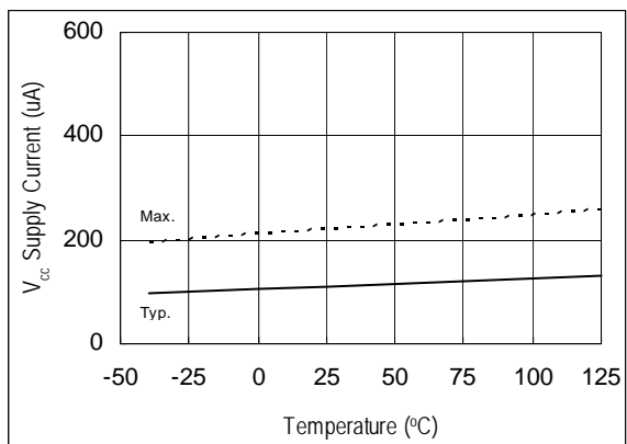
Figure 13A. V_{CC} Supply Current vs. Temperature
