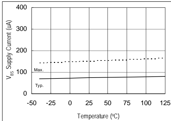
Figure 12A. V_{BS} Supply Current vs. Temperature
